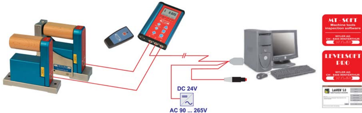
Set with BlueLEVEL BASIC and BlueMETER BASIC
